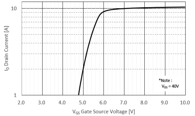
Figure 2. G_{FS} Characteristics
