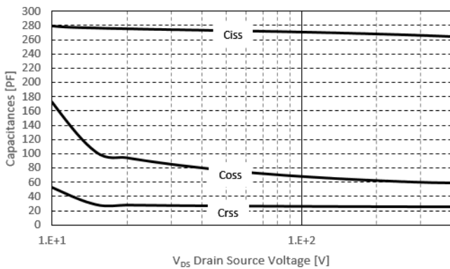
Figure 5. Capacitance Characteristics
